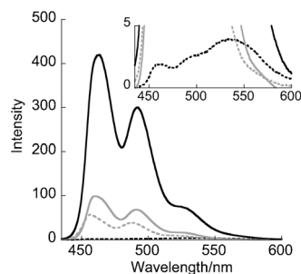
Figure 2. Fluorescence emission spectra of 1E 2 (gray) and 5E 2 -2 (black) in the presence (solid) and absence (dotted) of target Ds-ORN . Inset shows magnified spectra. Solution conditions were 1.0 \mu M probe, 2.0 \mu M Ds-ORN , 100 mM NaCl, 10 mM phosphate buffer, pH 7.0, 20 °C. Quantum yield of the probe/ Ds-ORN was listed in Table S1.
