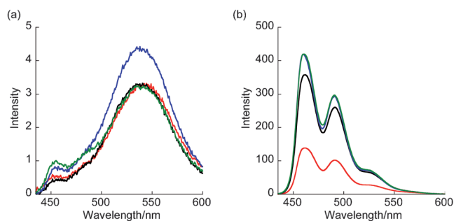
Figure 3. Fluorescent emission spectra of 8E 2 -2 (red), 6E 2 -2 (black), 6E 2 -3a (blue), and 6E 2 -3b (green) a) in the absence and b) presence of target Ds-ORN . Solution conditions were 1.0 \mu M probe, 2.0 \mu M Ds-ORN , 100 mM NaCl, 10 mM phosphate buffer, pH 7.0, 20 °C. Quantum yields of the probe/ Ds-ORN were listed in Table S1.
